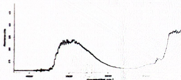
Infrared Spectrum 红外光谱
